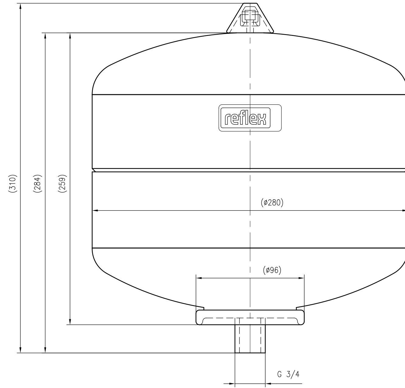
Front view
