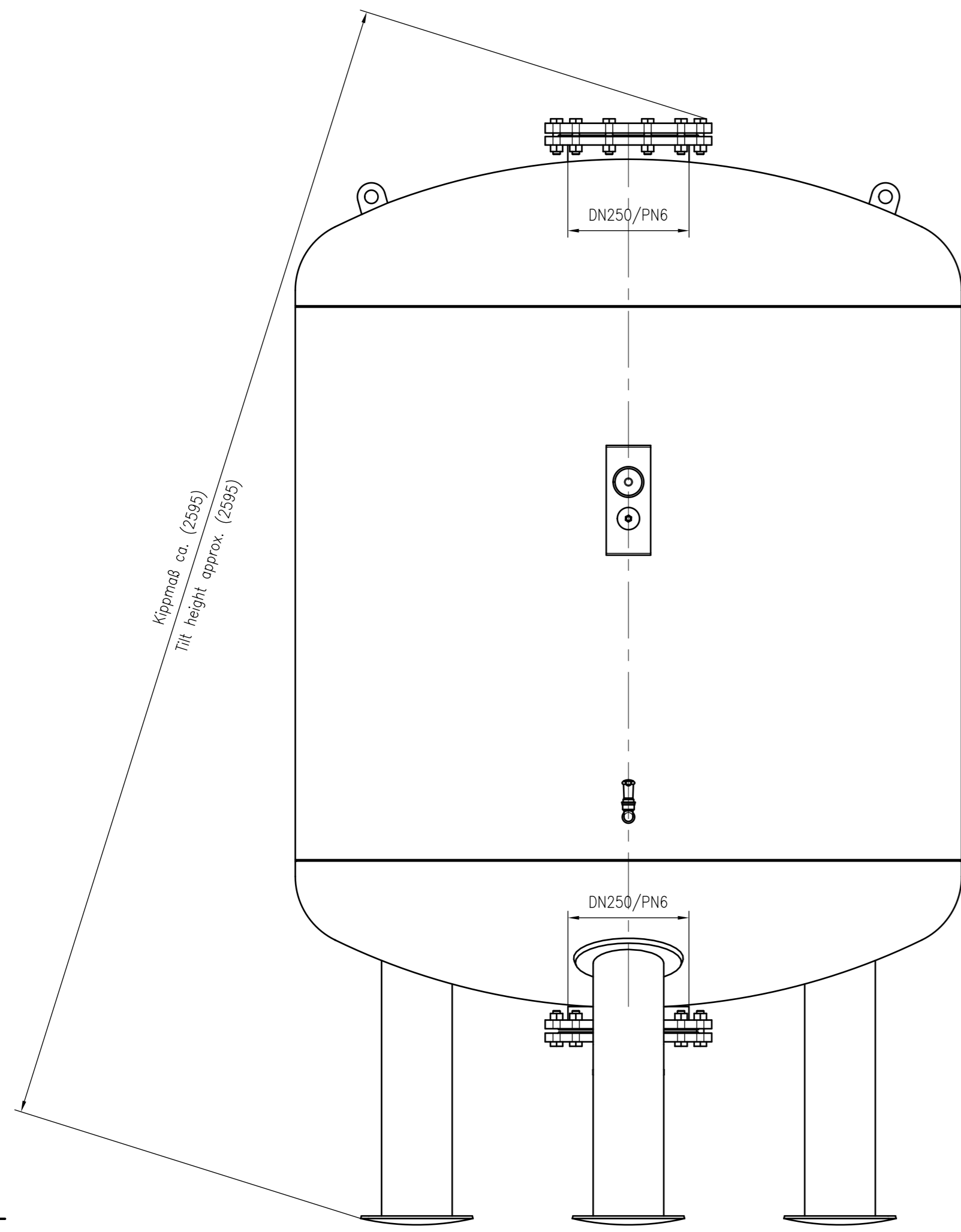
Side view
