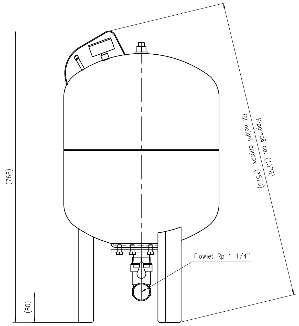
Side view
