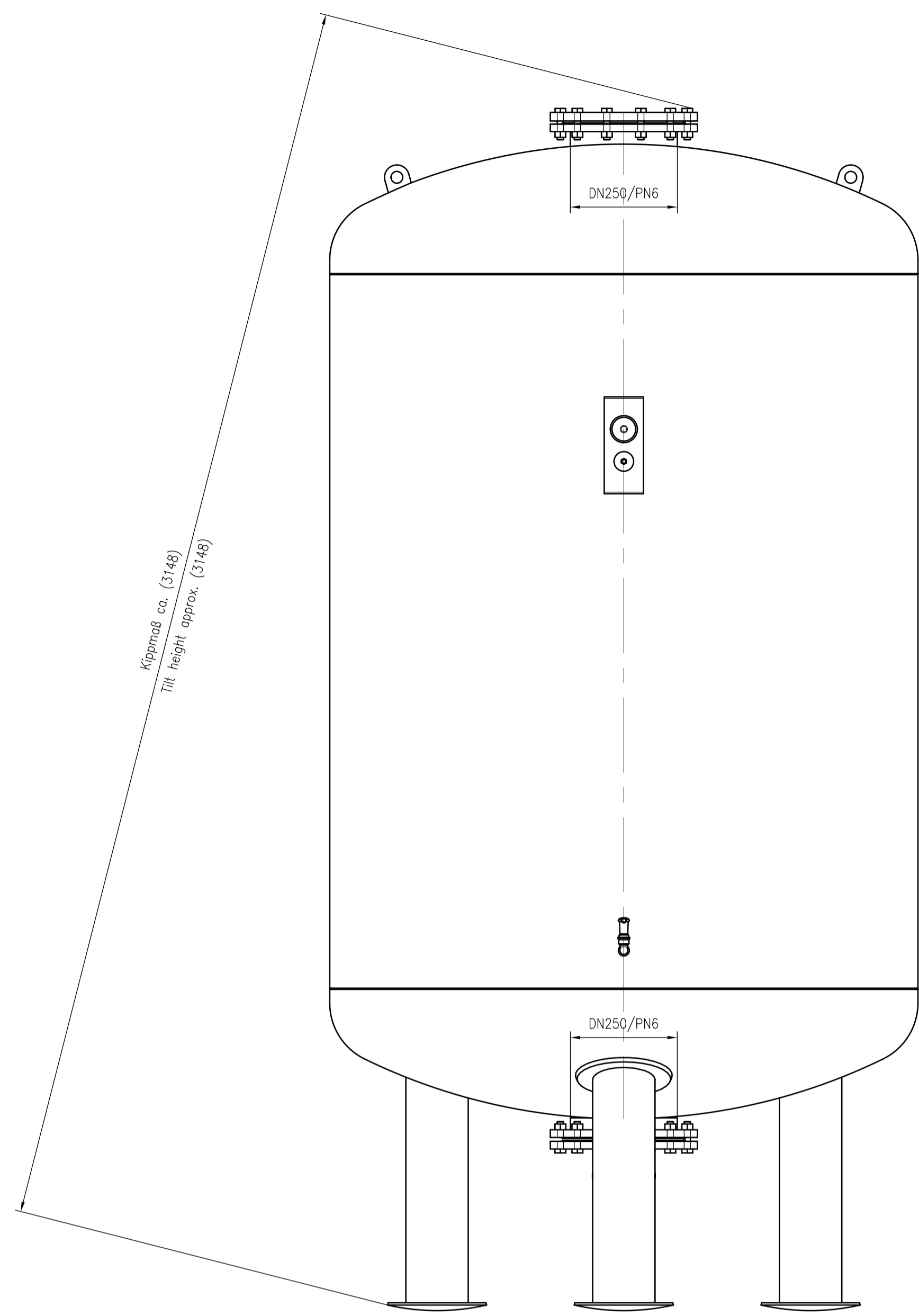
Side view
