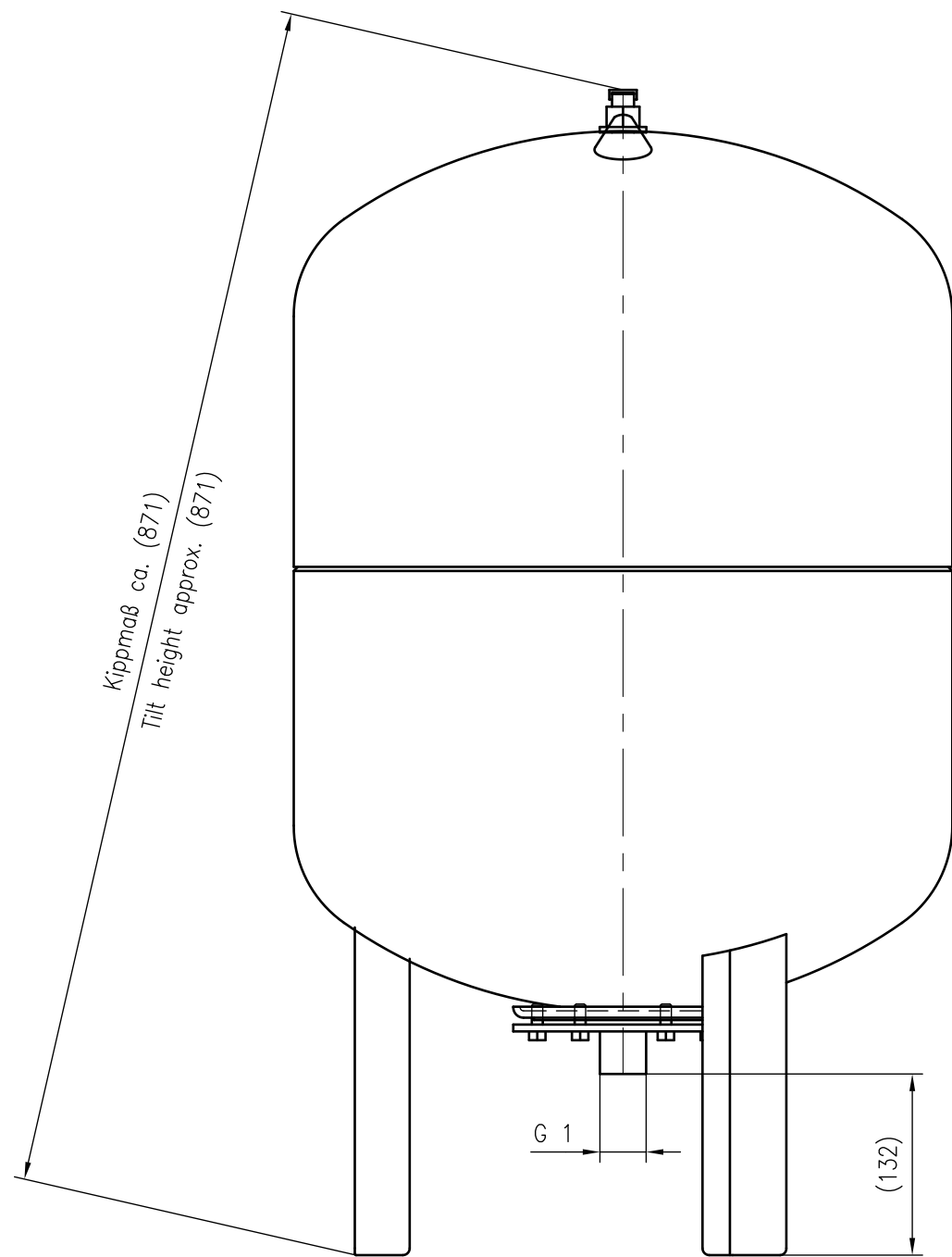
Side view
