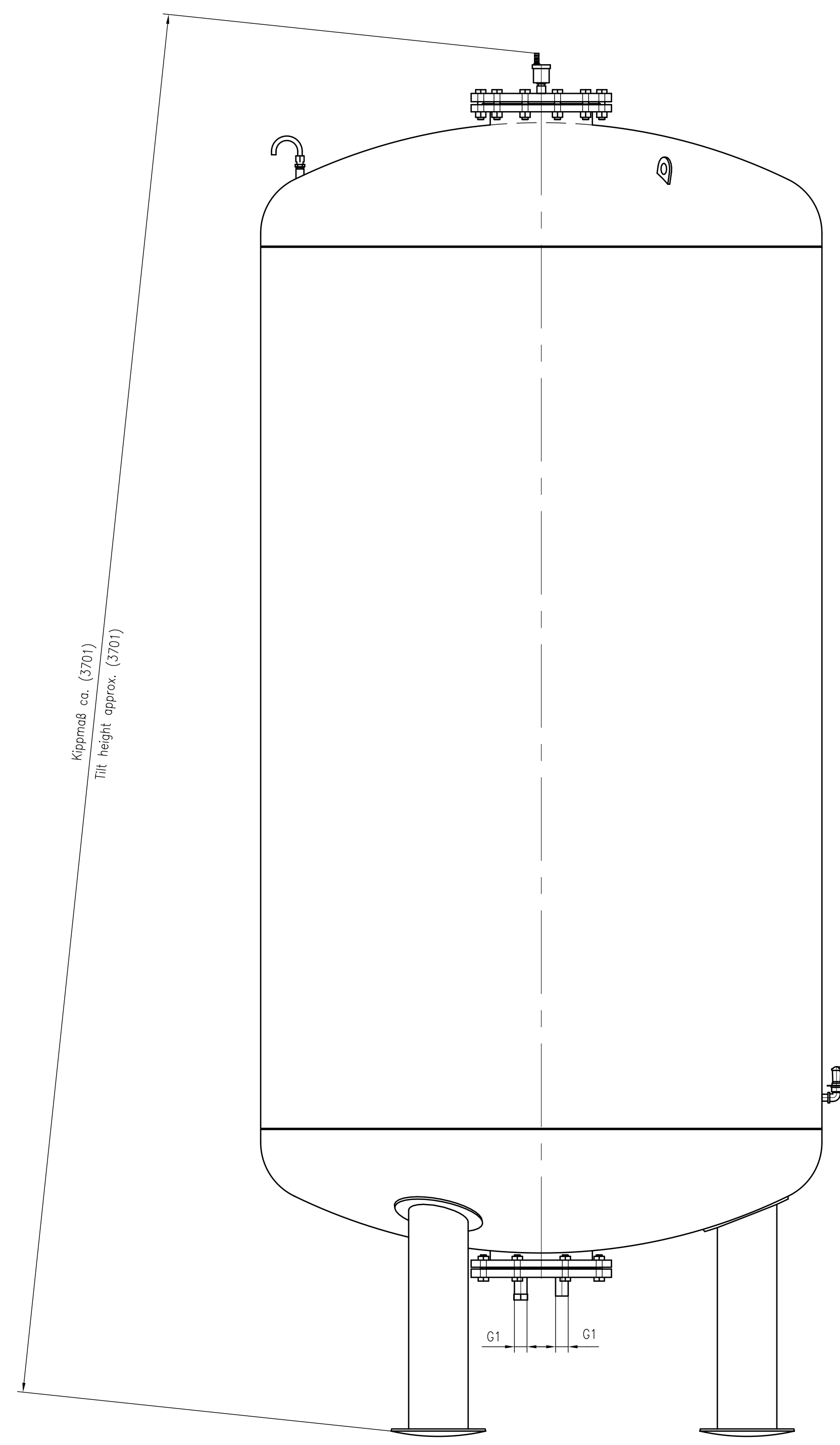
Side view
