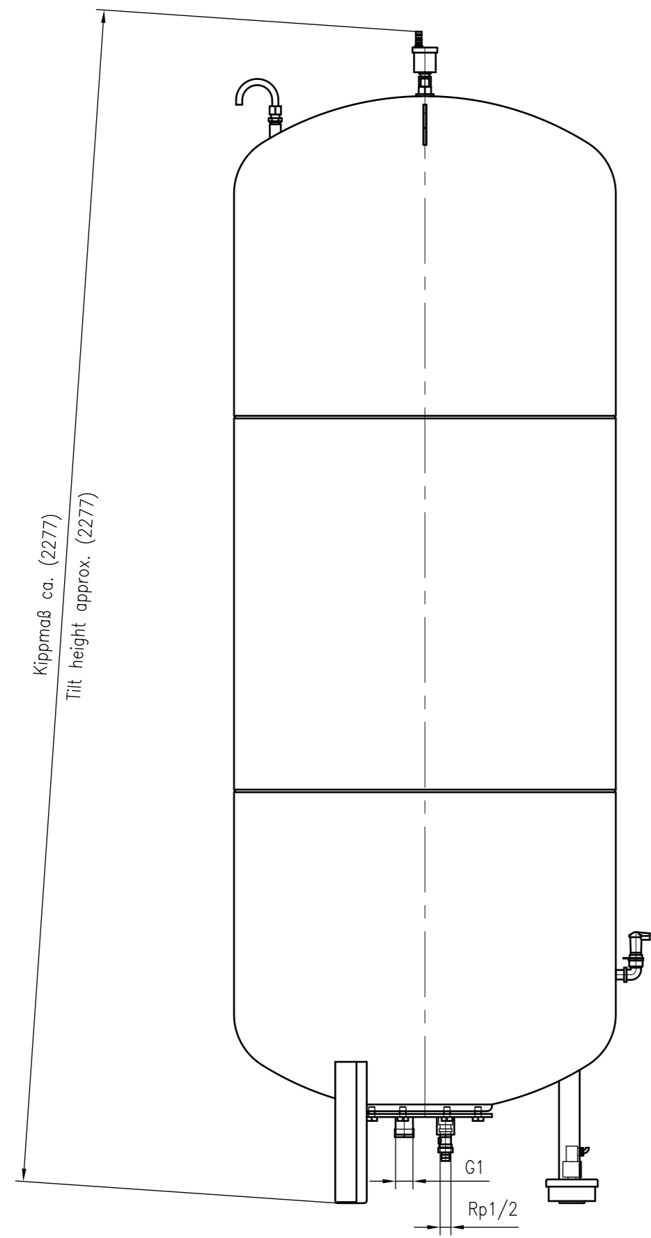
Side view
