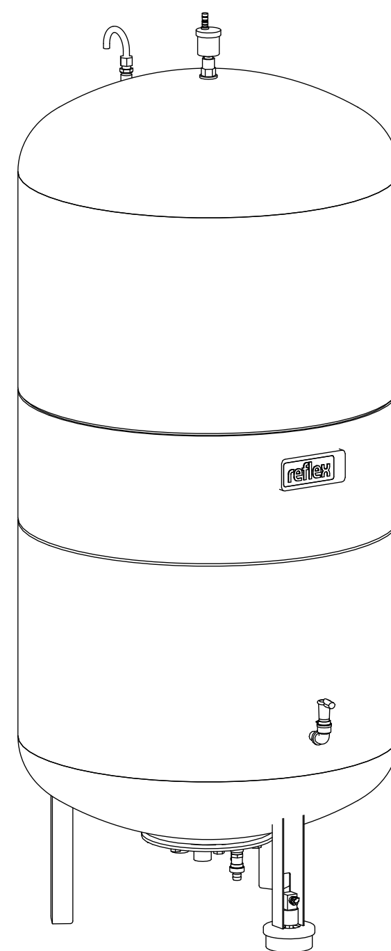
Isometric view
