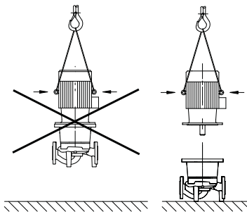
Fig. 7: Transport silnika
